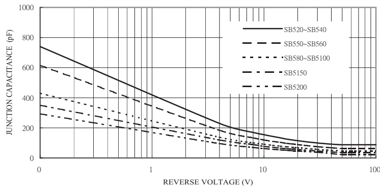
FIG. 4-TYPICAL JUNCTION CAPACITANCE
