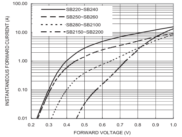
FIG. 2-TYPICAL FORWARD CHARACTERISTICS
